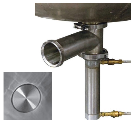
3" Air Piston Valve with Acme Thread (Kettle bottom with valve in closed position)
